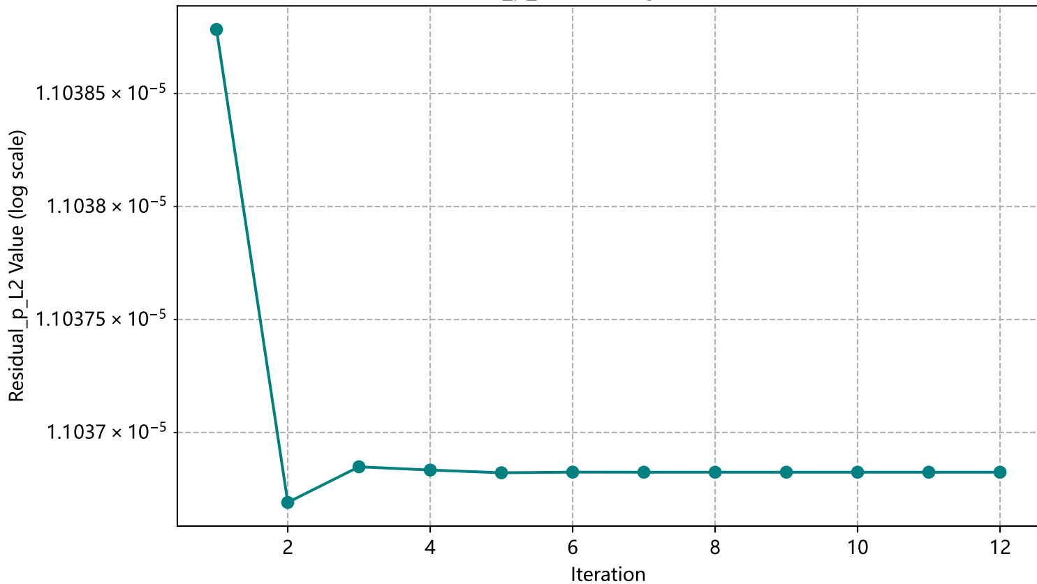
Residual_p_L2 Convergence (Va=0.9)
