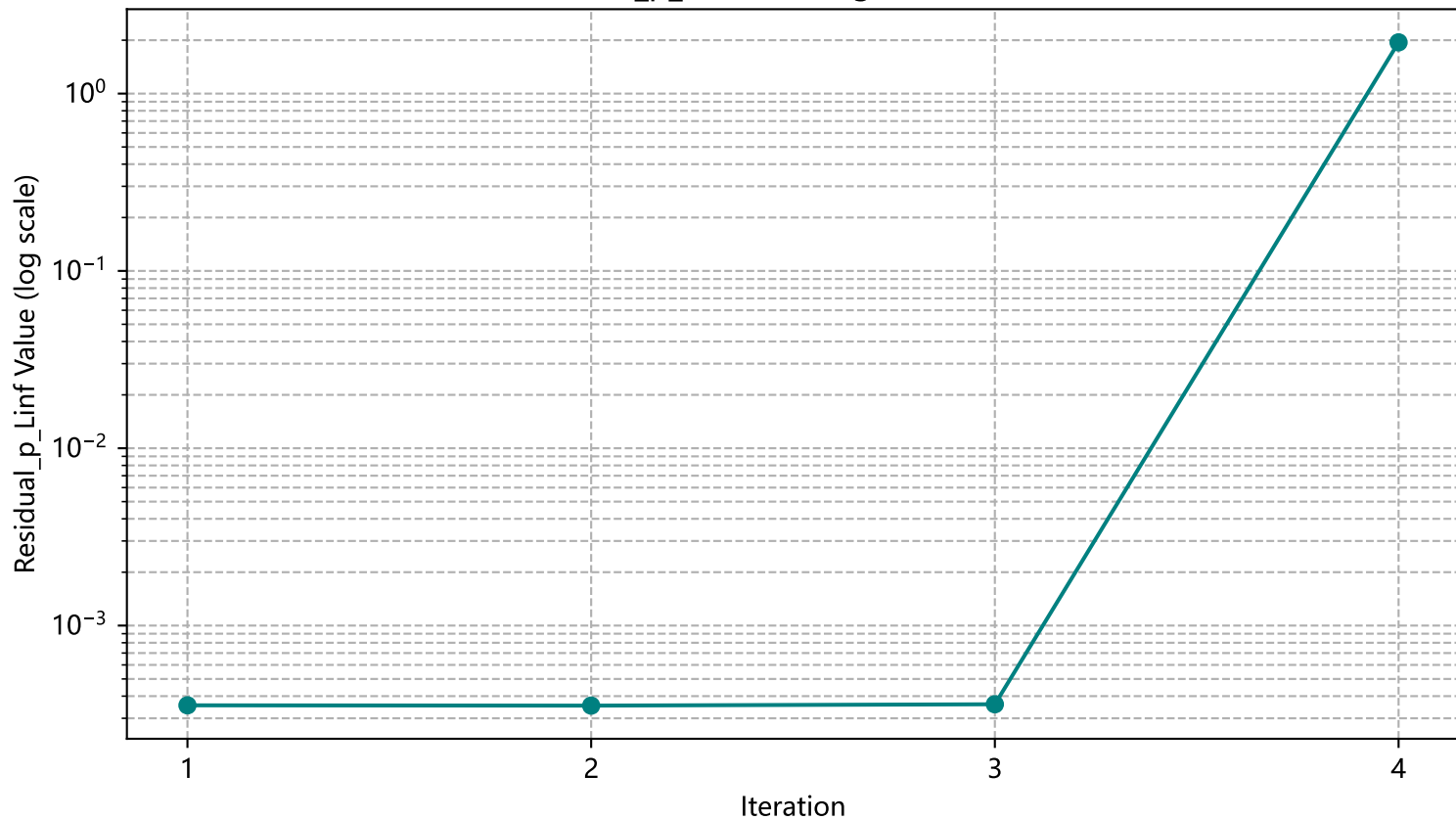
Residual_p_Linf Convergence (Va=1.1)
