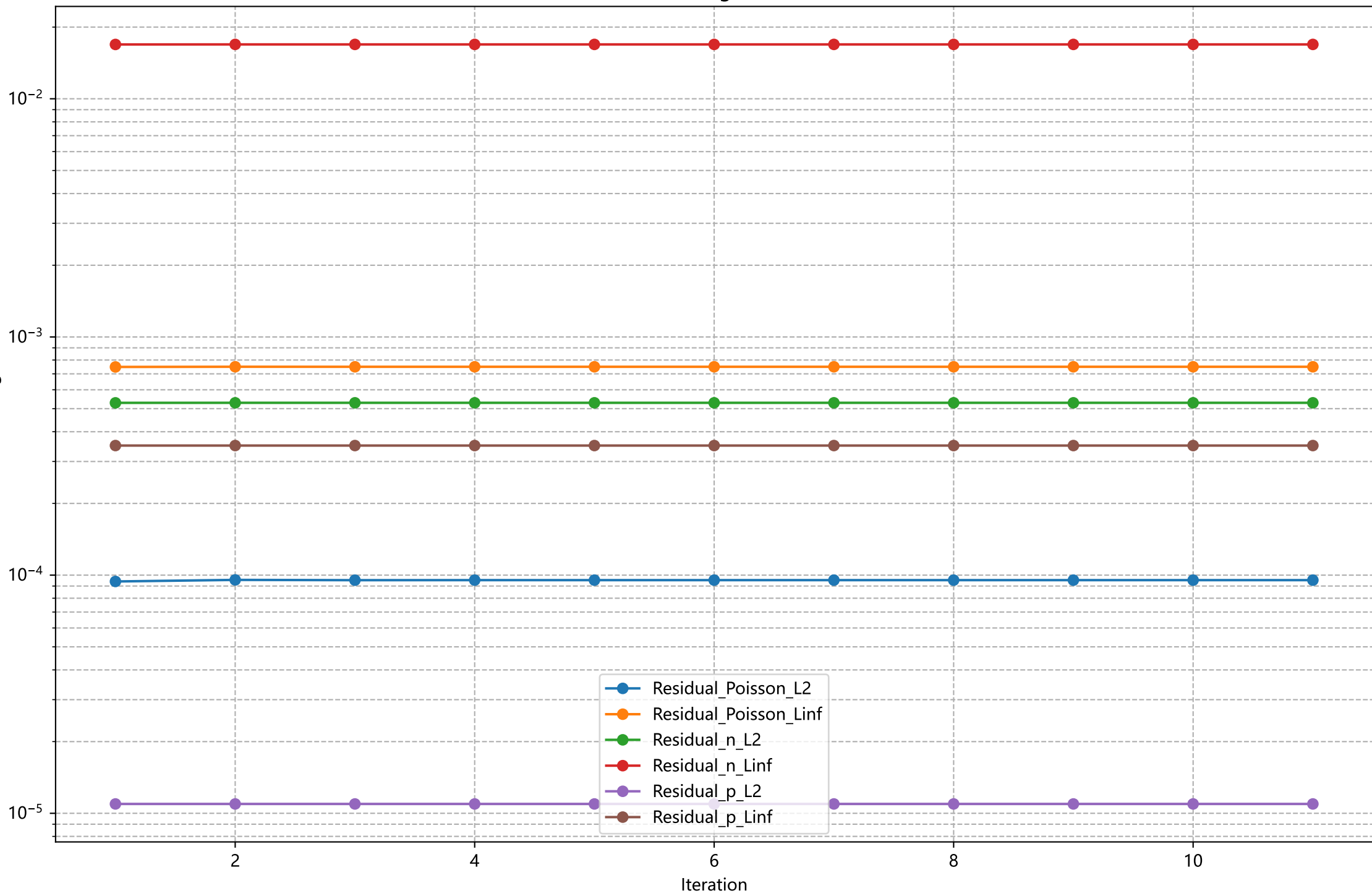
Residual Convergence (Va=0.5)
