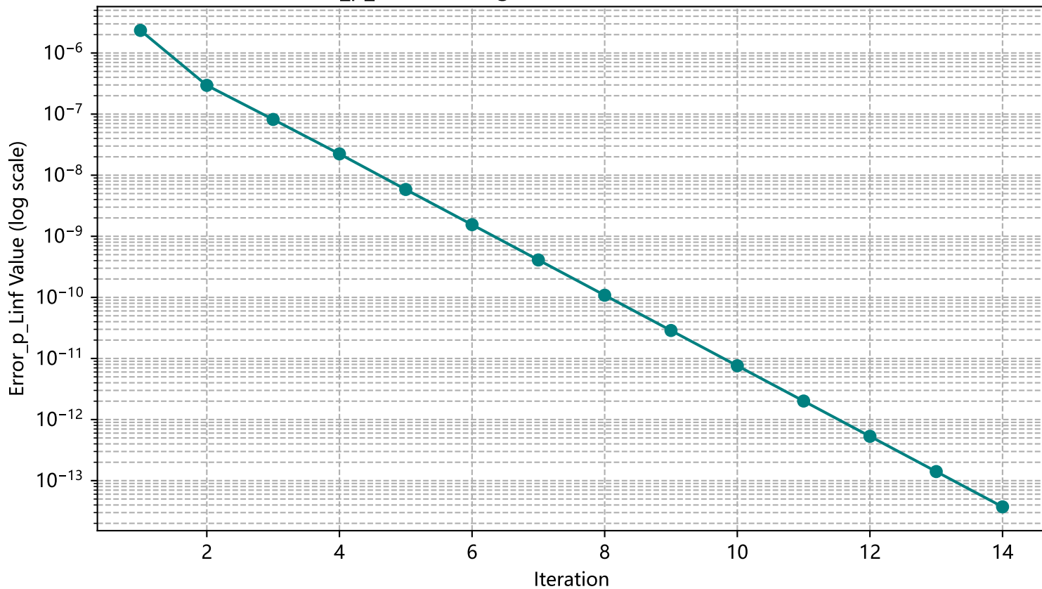
Error_p_Linf Convergence (Va=0.6000000000000001)
