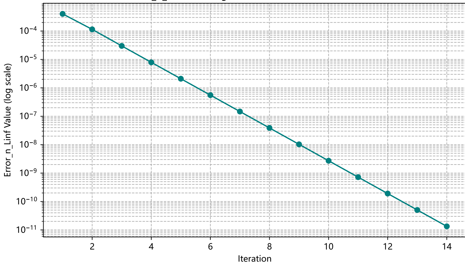
Error_n_Linf Convergence (Va=0.6000000000000001)
