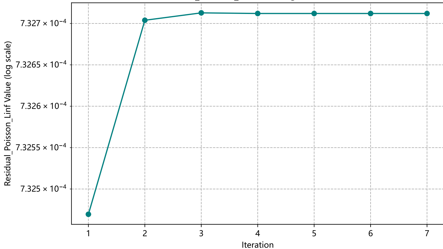
Residual_Poisson_Linf Convergence (Va=0.1)
