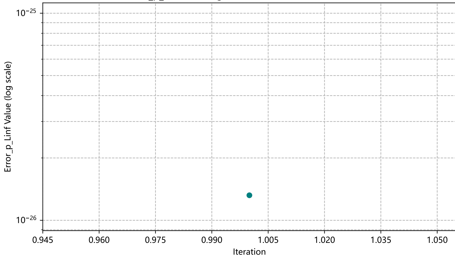
Error_p_Linf Convergence (Va=1.2000000000000002)
