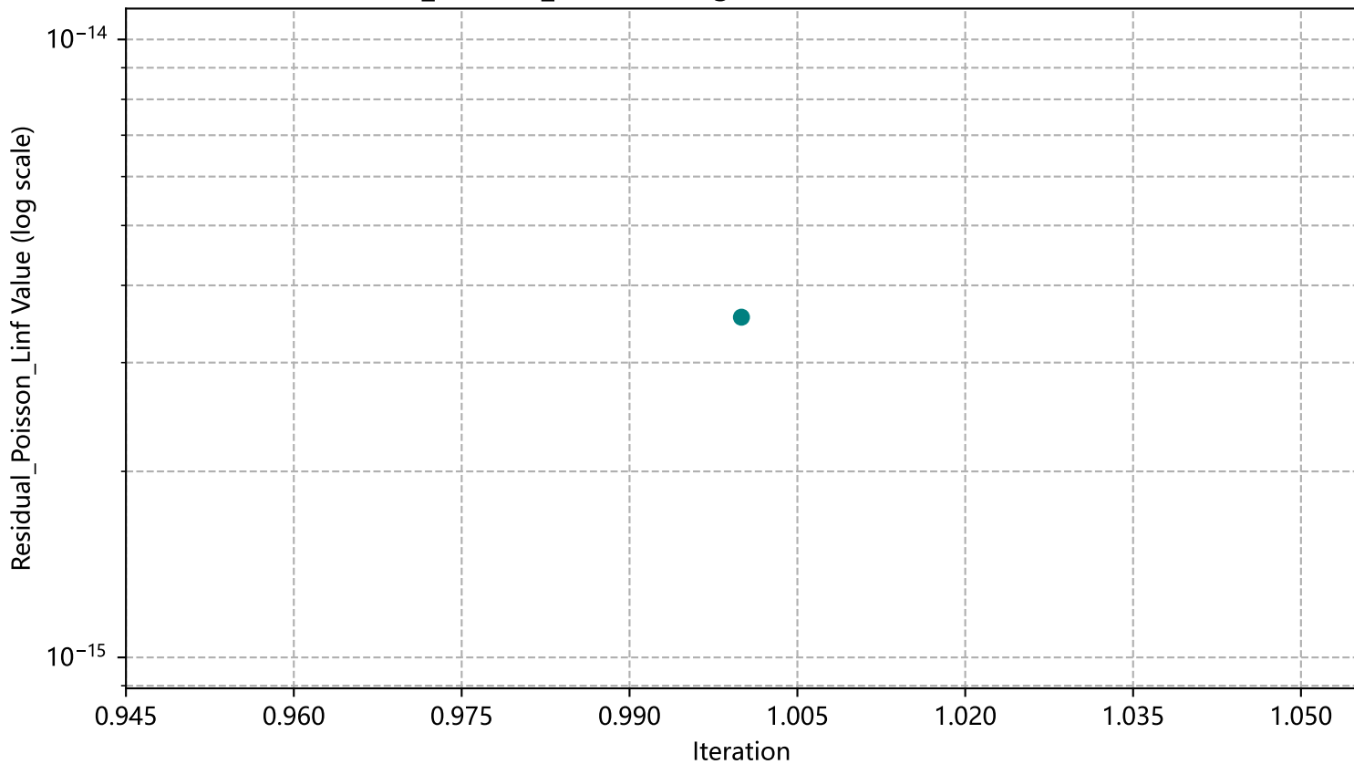
Residual_Poisson_Linf Convergence (Va=0.7000000000000001)
