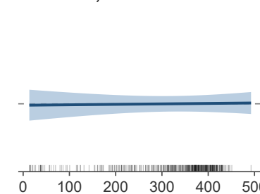
Distance SD, near zone (m) edf = 0.24, n.s.
