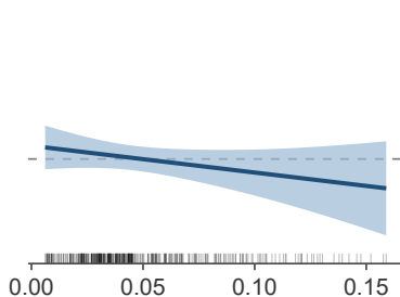
NDVI variance edf = 1.02, p < 0.01
