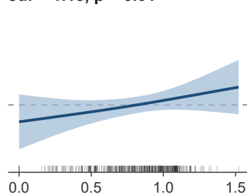
Vertical structural heterogeneity edf = 1.13, p < 0.01
