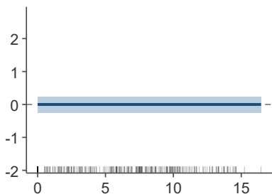
Forest ecotone density edf = 0.00, n.s.
