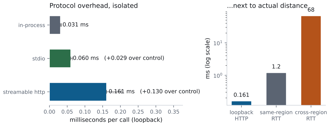
Figure 3.2 Left: protocol overhead with server execution subtracted out. Right: the same numbers next to actual network distance, on a log scale, which is the honest context.
