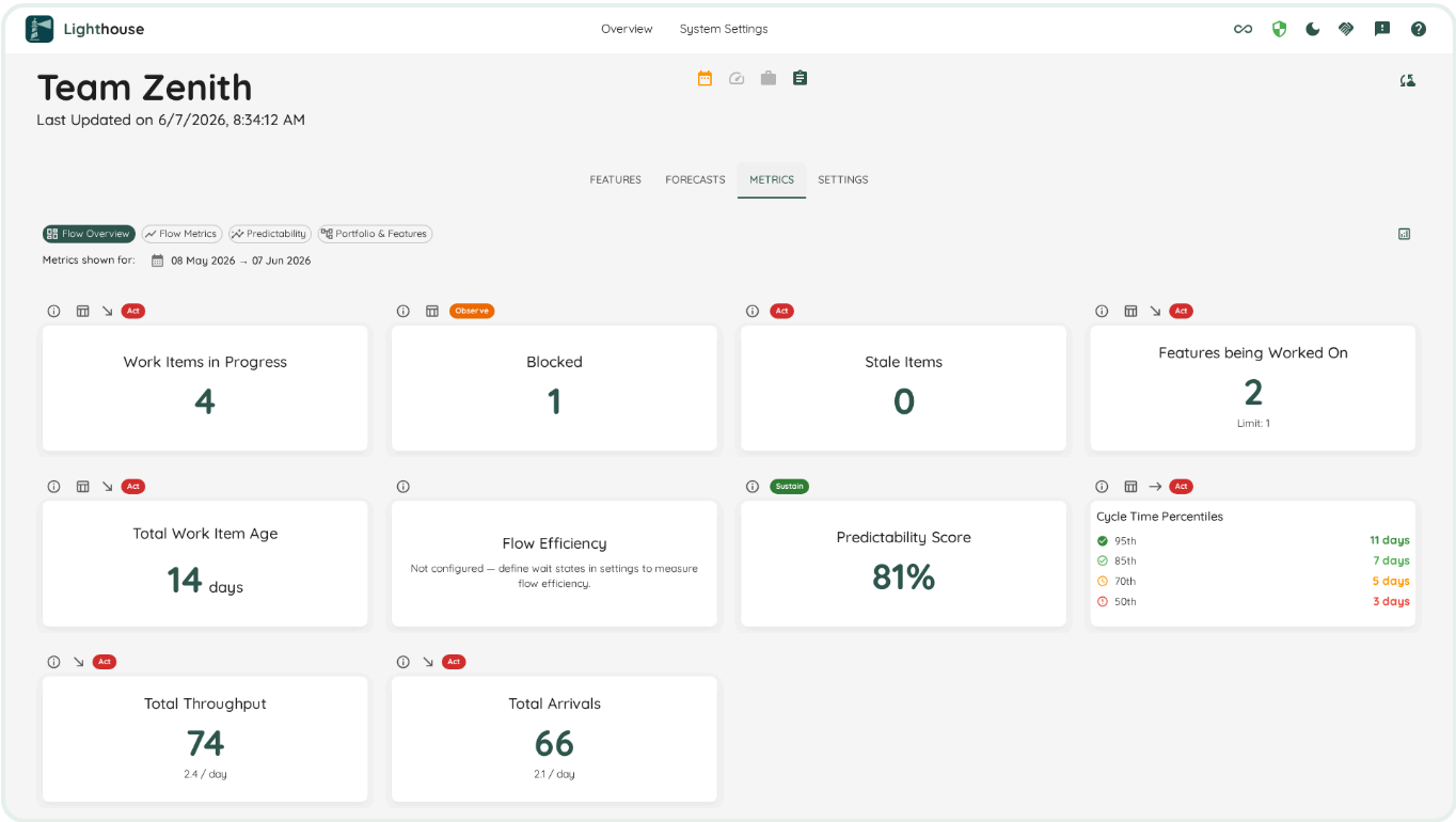
The Lighthouse metrics dashboard, fully customisable per team.
