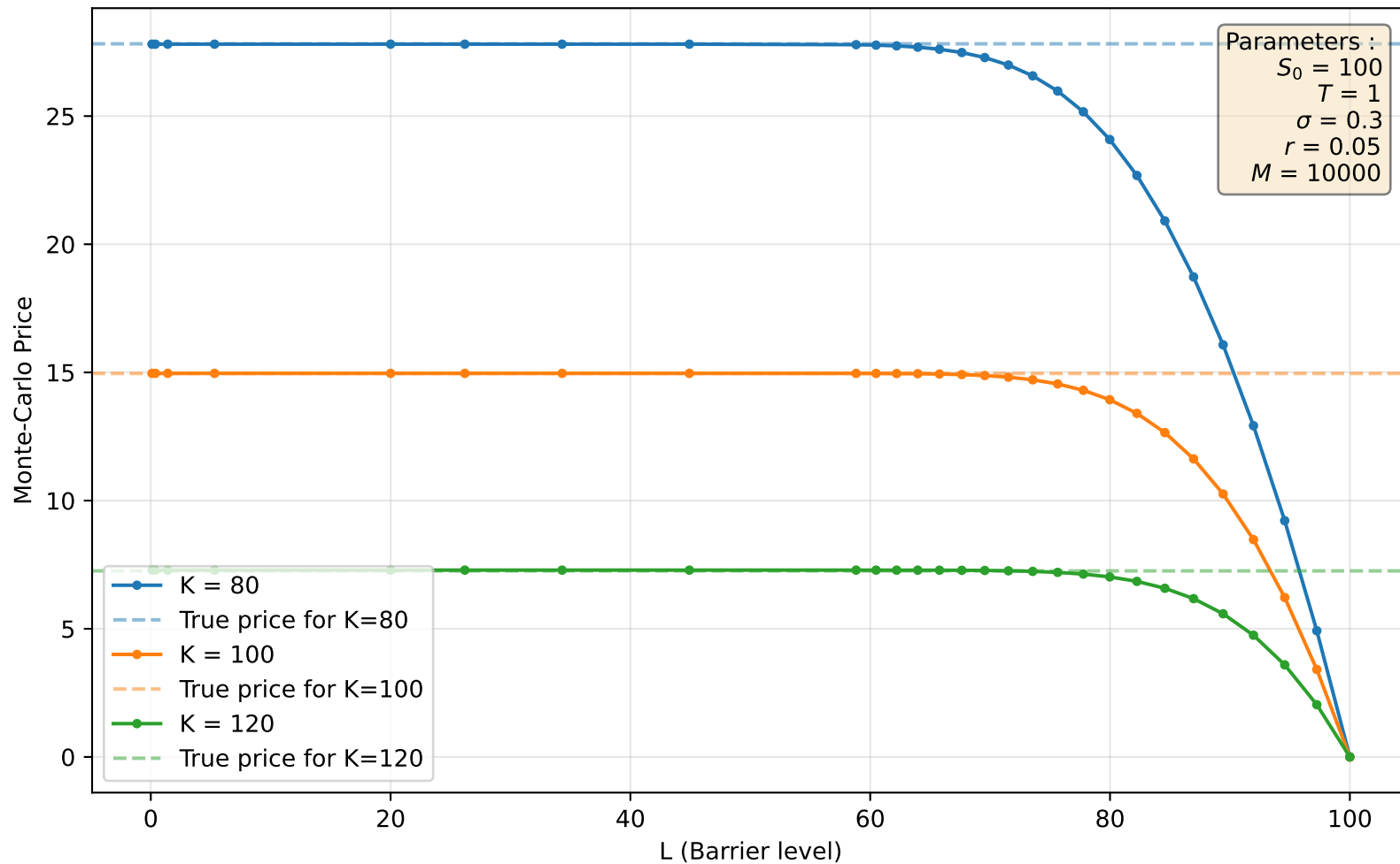
Barrier Call Price vs European call true price
