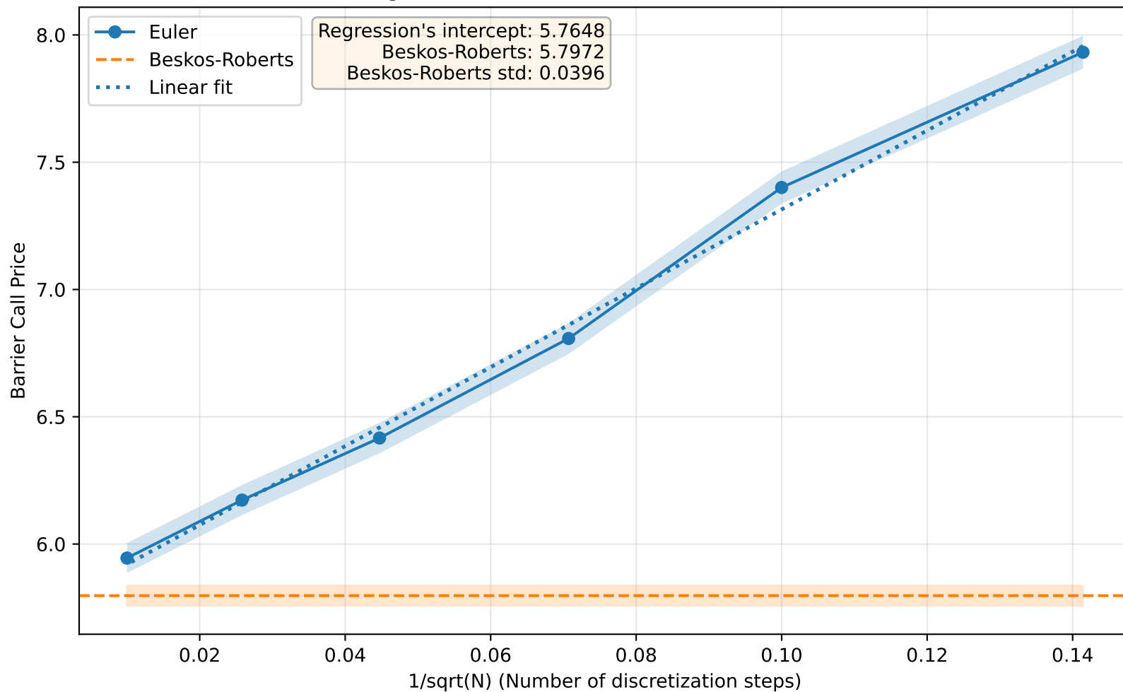
Convergence: Euler Discretization vs Beskos-Roberts
