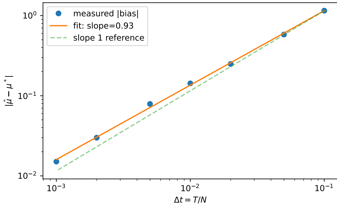
Euler weak convergence: BS, r=0.4 , \sigma=0.1
