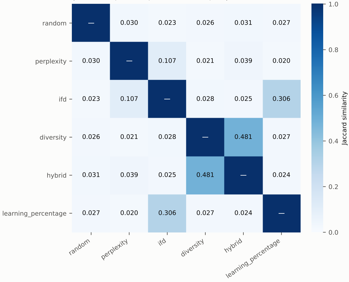
Pairwise Jaccard similarity between selections (ratio=0.05, seed=0, k=700 from 14,000)
