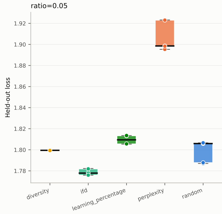
Held-out loss across seeds per method (lower spread = more stable)
