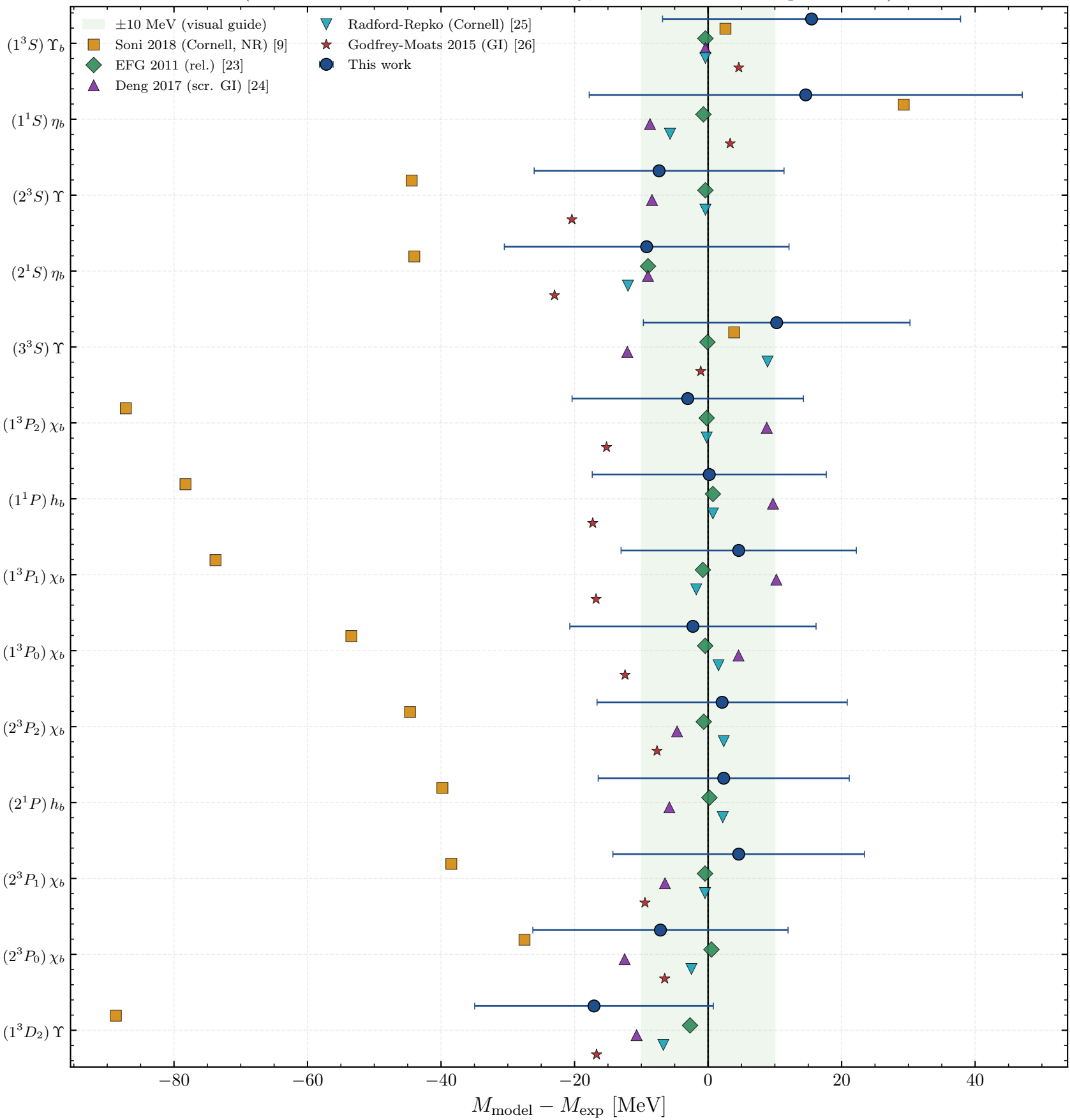
Bottomonium bb : Hamiltonian vs. literature (this work's bars = model uncertainty; literature values are predictions)
