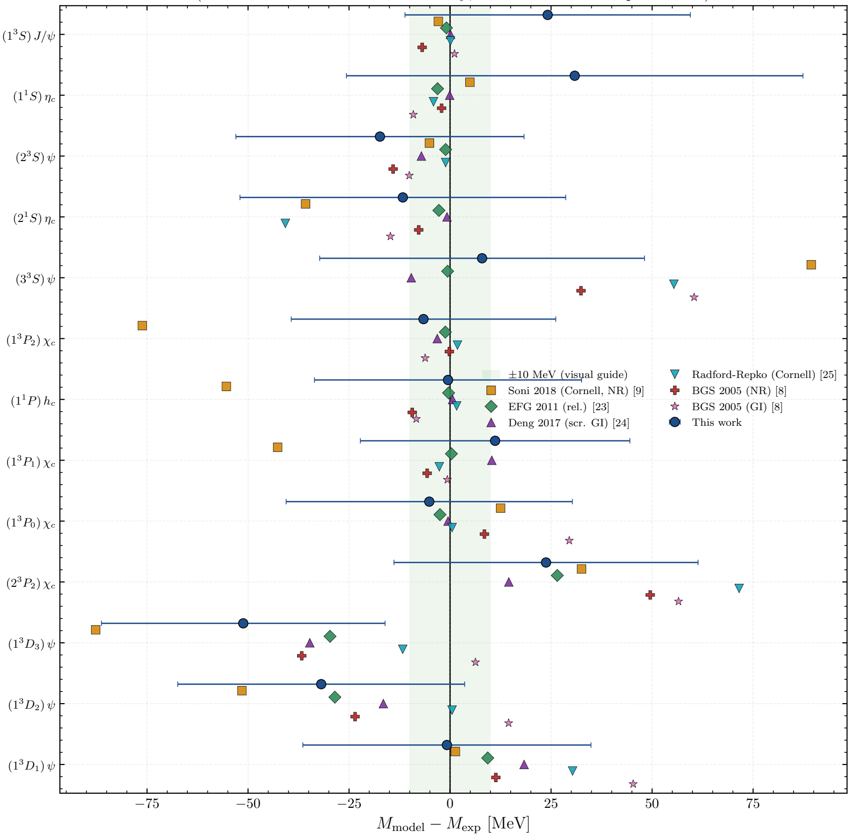
Charmonium c\bar{c} : Hamiltonian vs. literature (this work's bars = model uncertainty; literature values are predictions)
