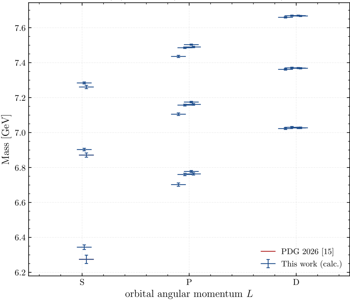
B_c ( b\bar{c} ) spectrum (bars: model uncertainty)
