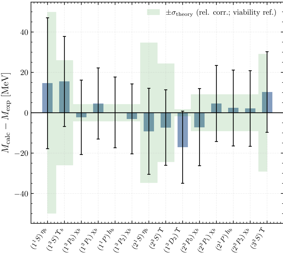
Bottomonium b\bar{b} mass residuals (bars: computational \sigma ; band: \sigma_{\text{theory}} ref.) Charmonium c\bar{c} mass residuals (bars: computational \sigma ; band: \sigma_{\text{theory}} ref.)
