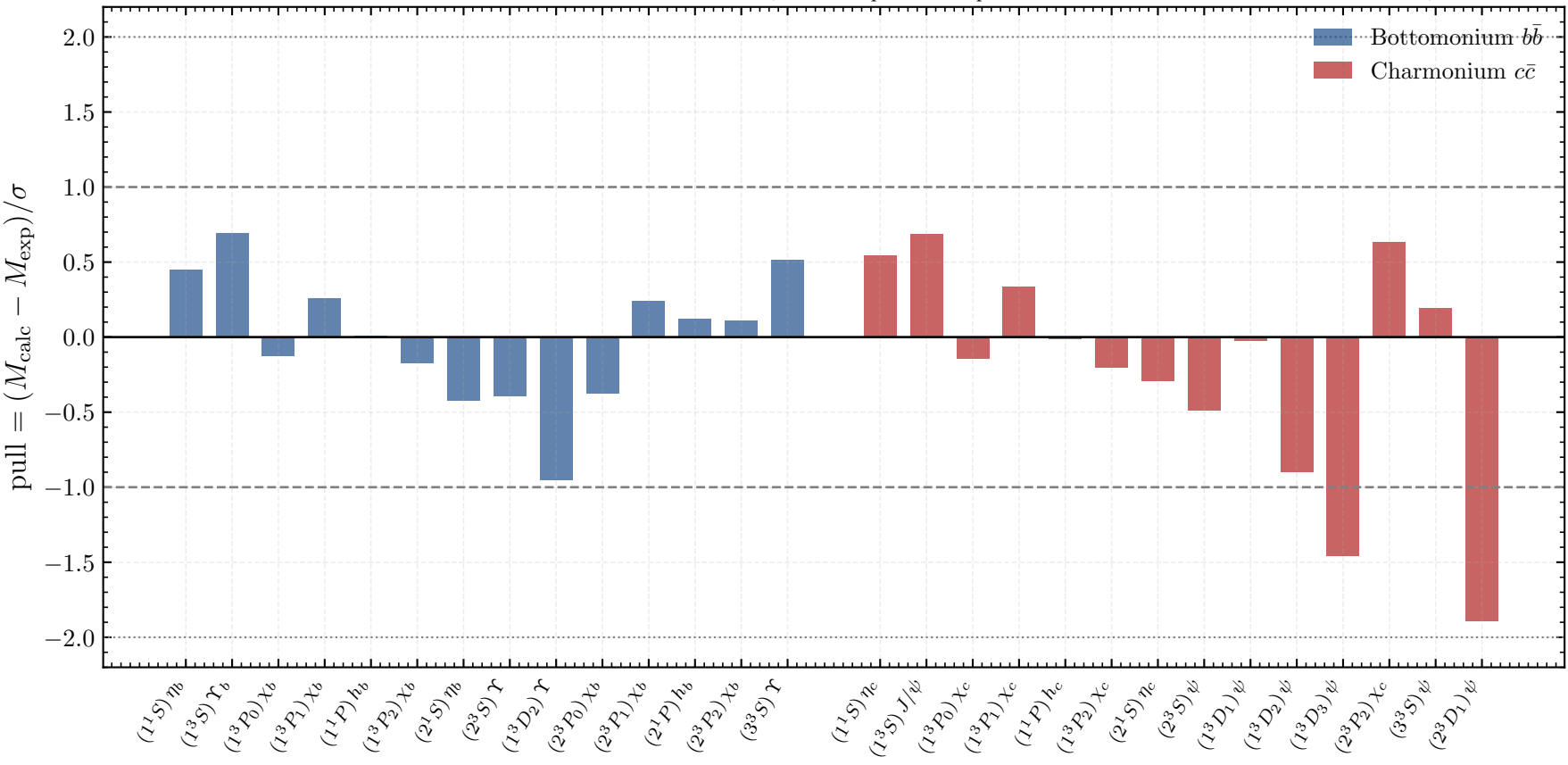
Mass pulls vs. computational uncertainty ( \sigma = \sigma_{\text{exp}} \oplus \sigma_{\text{comp}} , propagated parameter covariance)
