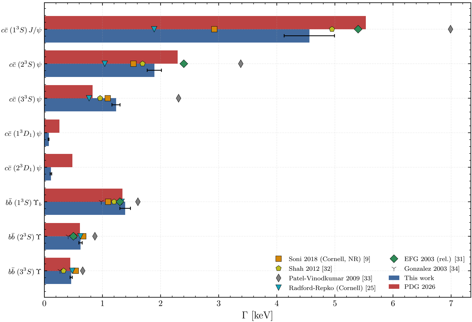
Leptonic V \rightarrow e^+e^- widths vs. PDG and literature
