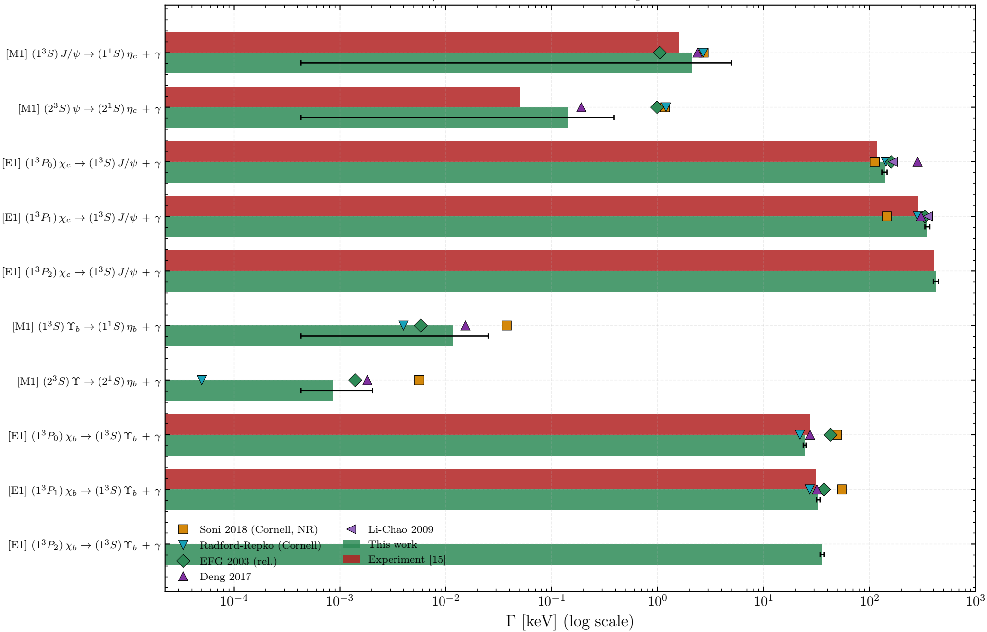
Radiative E1/M1 transition widths vs. experiment and literature
