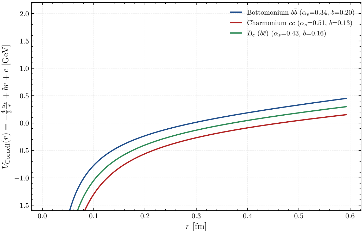
Fitted Cornell potentials by sector
