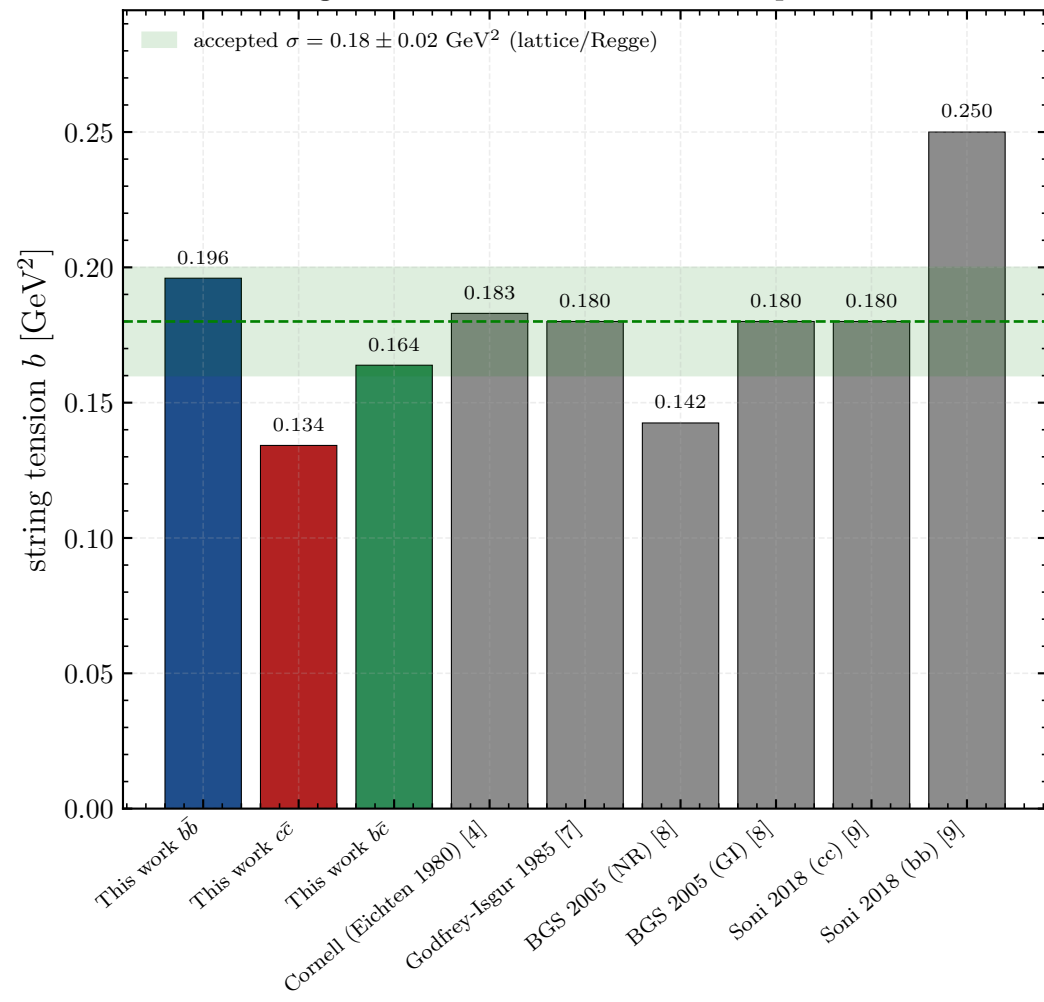
String tension vs. literature and accepted value
