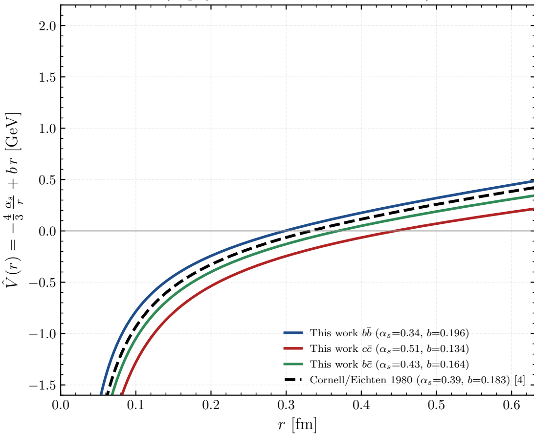
Cornell potential shape vs. the canonical form (unphysical constant offset c removed)
