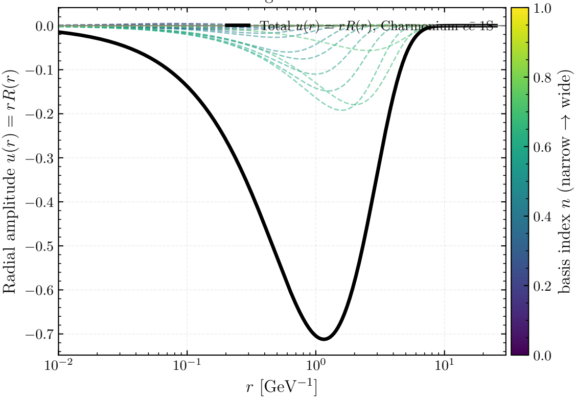
GEM basis coverage: Charmonium c\bar{c} 1S
