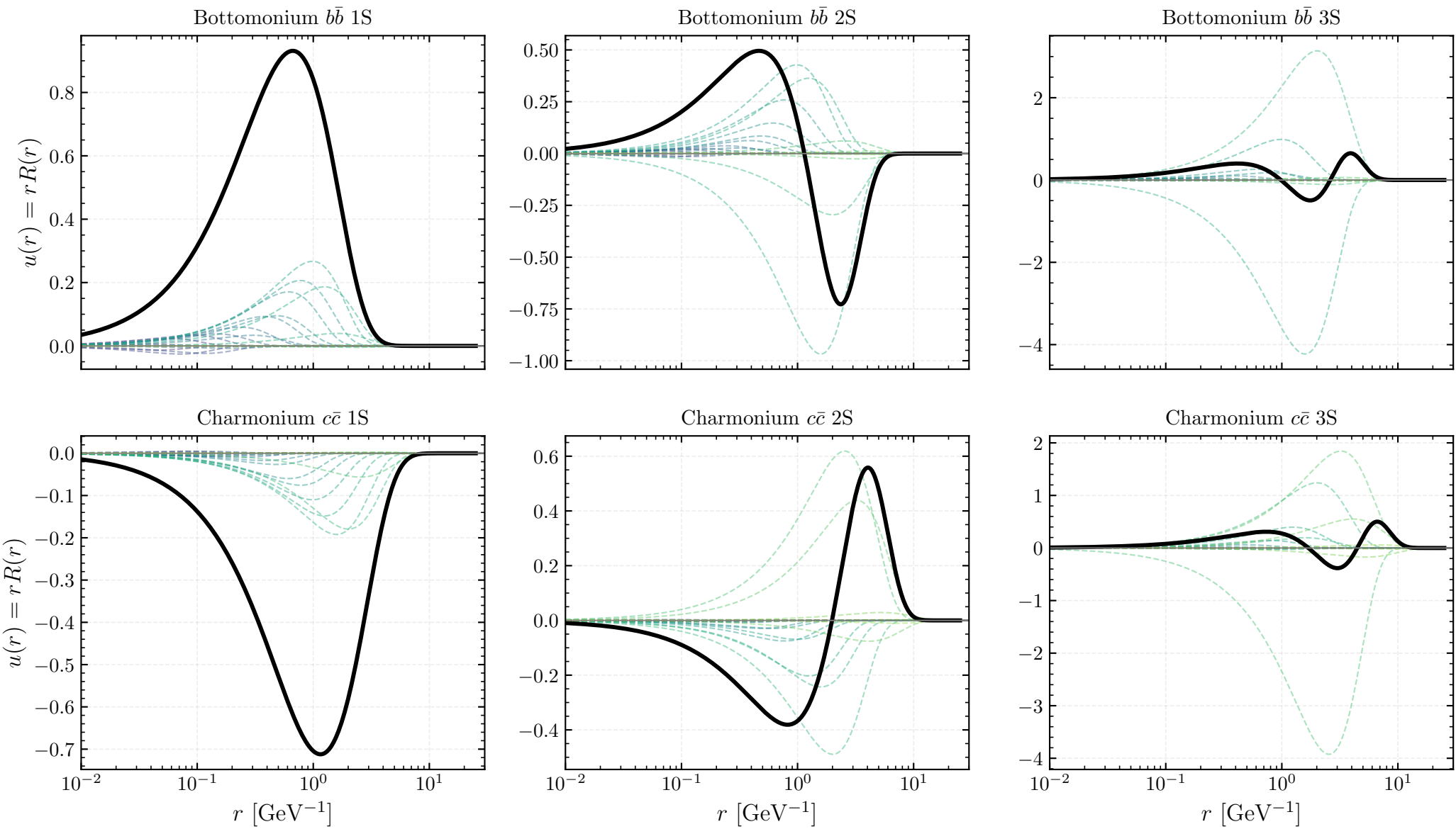
GEM basis-function coverage of the radial wavefunctions (dashed: weighted Gaussians, solid: total)
