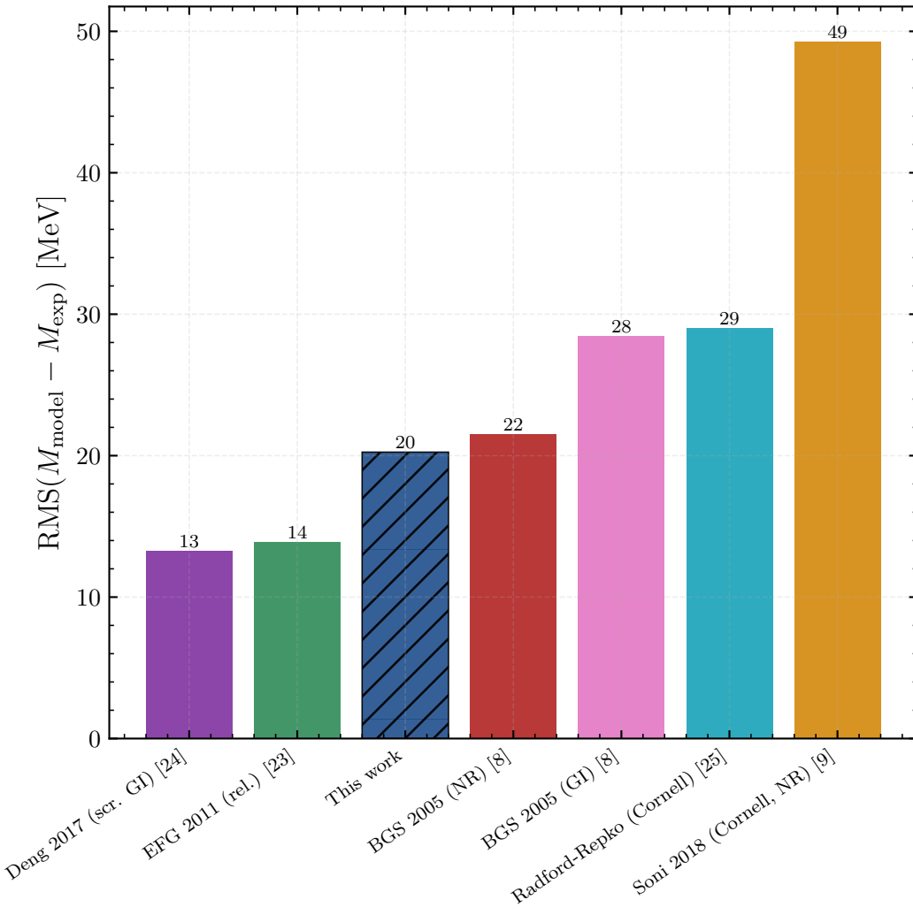
Charmonium c\bar{c} ( N = 13 common states)
