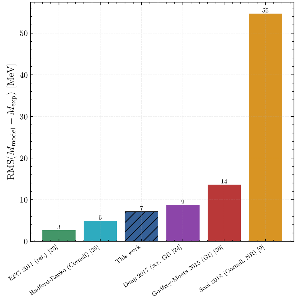
Bottomonium b\bar{b} ( N = 13 common states)
