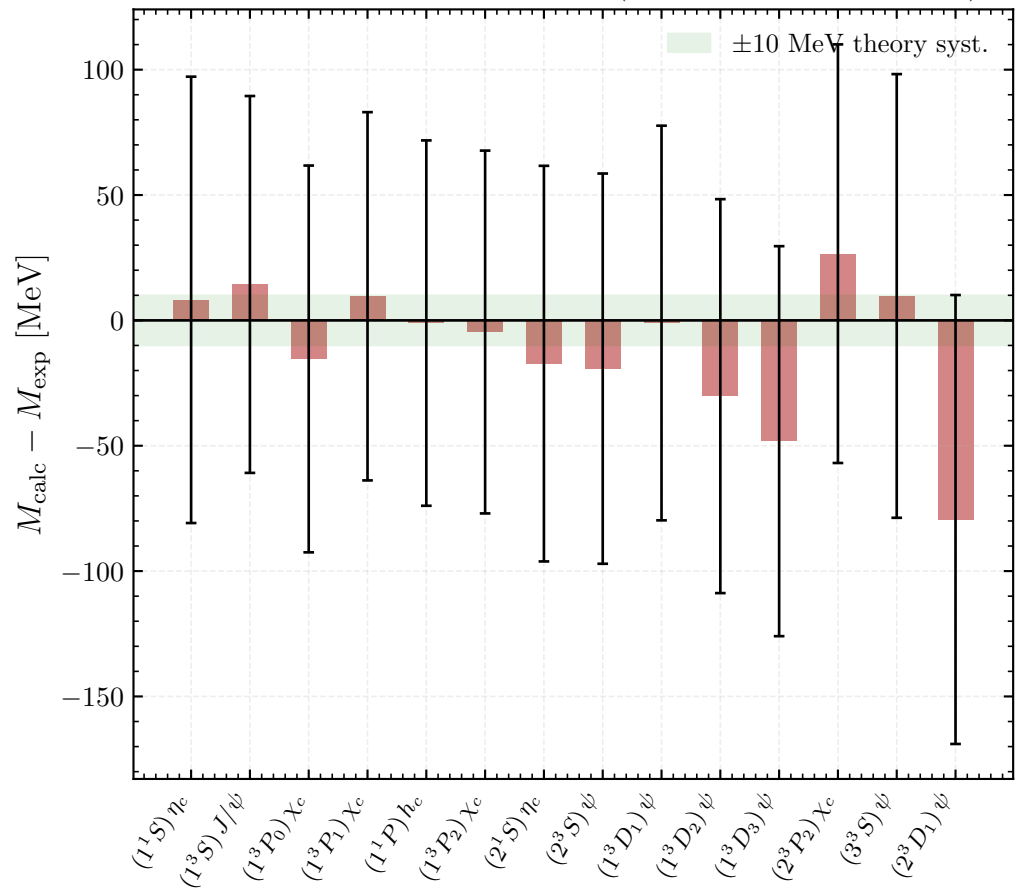
Charmonium c\bar{c} mass residuals (bars: model uncertainty)
