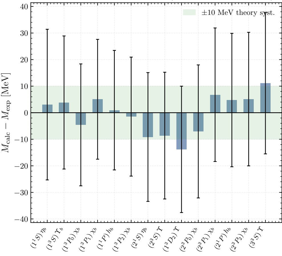
Bottomonium b\bar{b} mass residuals (bars: model uncertainty)
