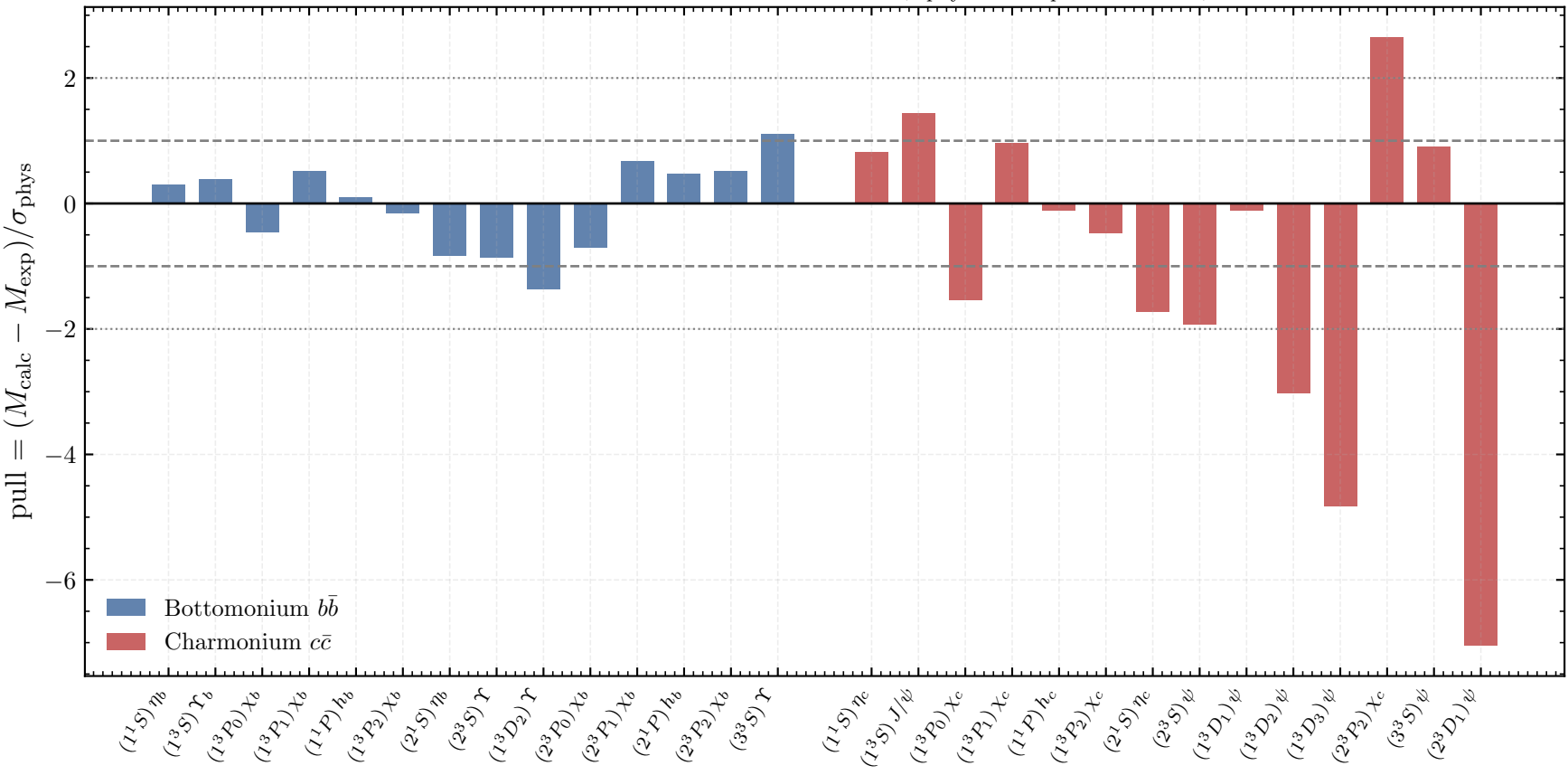
Mass pulls vs. physical uncertainty ( \sigma_{\text{phys}} = \sigma_{\text{exp}} \oplus 10 \text{ MeV} )
