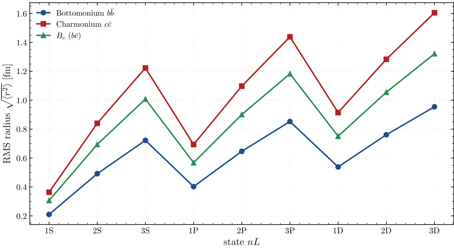
RMS radii: tighter binding for heavier systems
