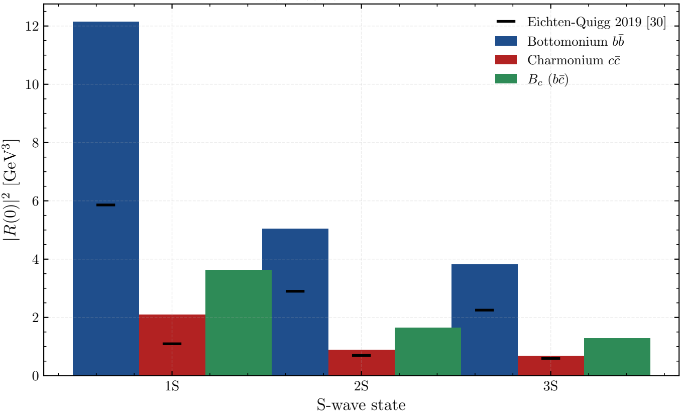
Wavefunction at the origin |R(0)|^2 (bars: this work; ticks: Eichten-Quigg 2019)
