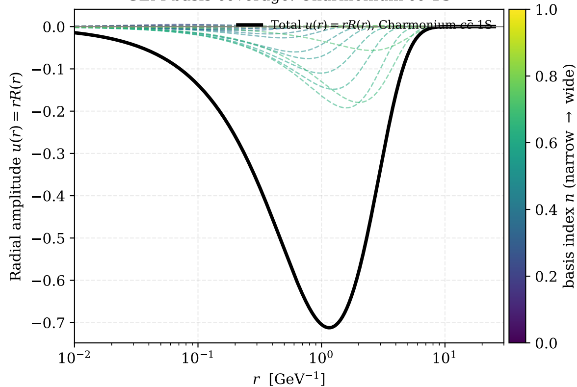
GEM basis coverage: Charmonium c\bar{c} 1S
