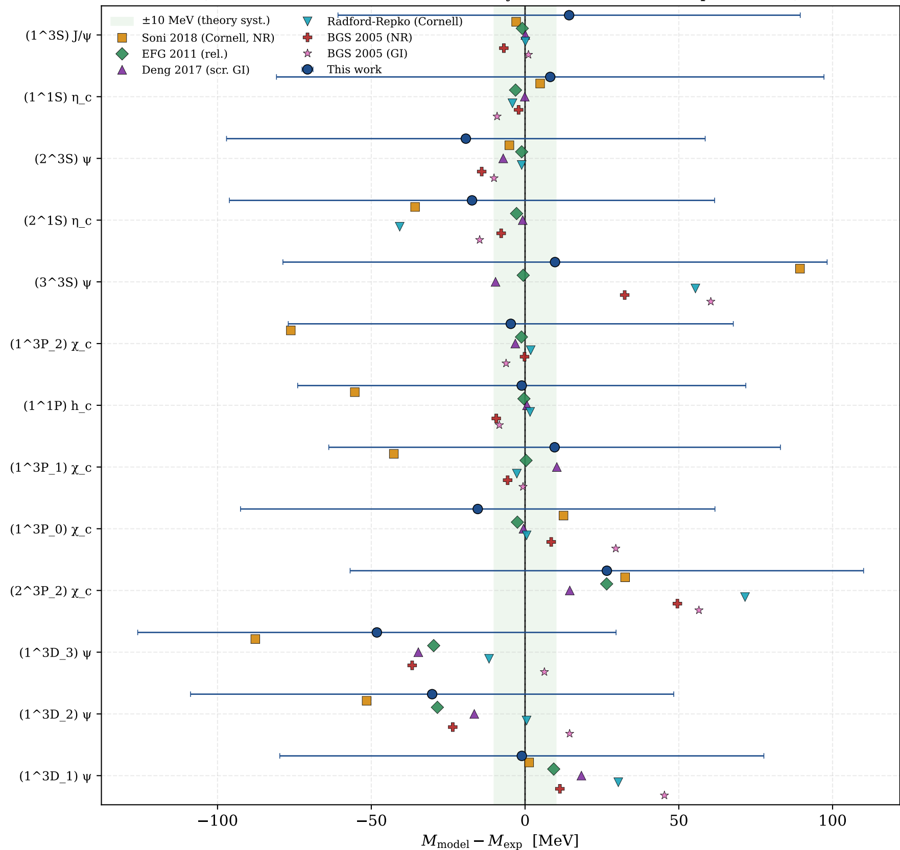
Charmonium c\bar{c} : Hamiltonian vs. literature (this work's bars = model uncertainty; literature values are predictions)
