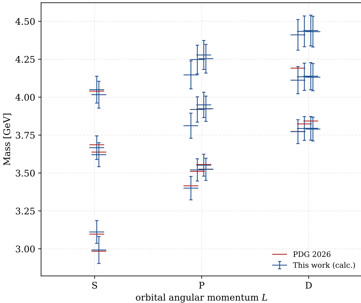
Charmonium c\bar{c} spectrum (bars: model uncertainty)
