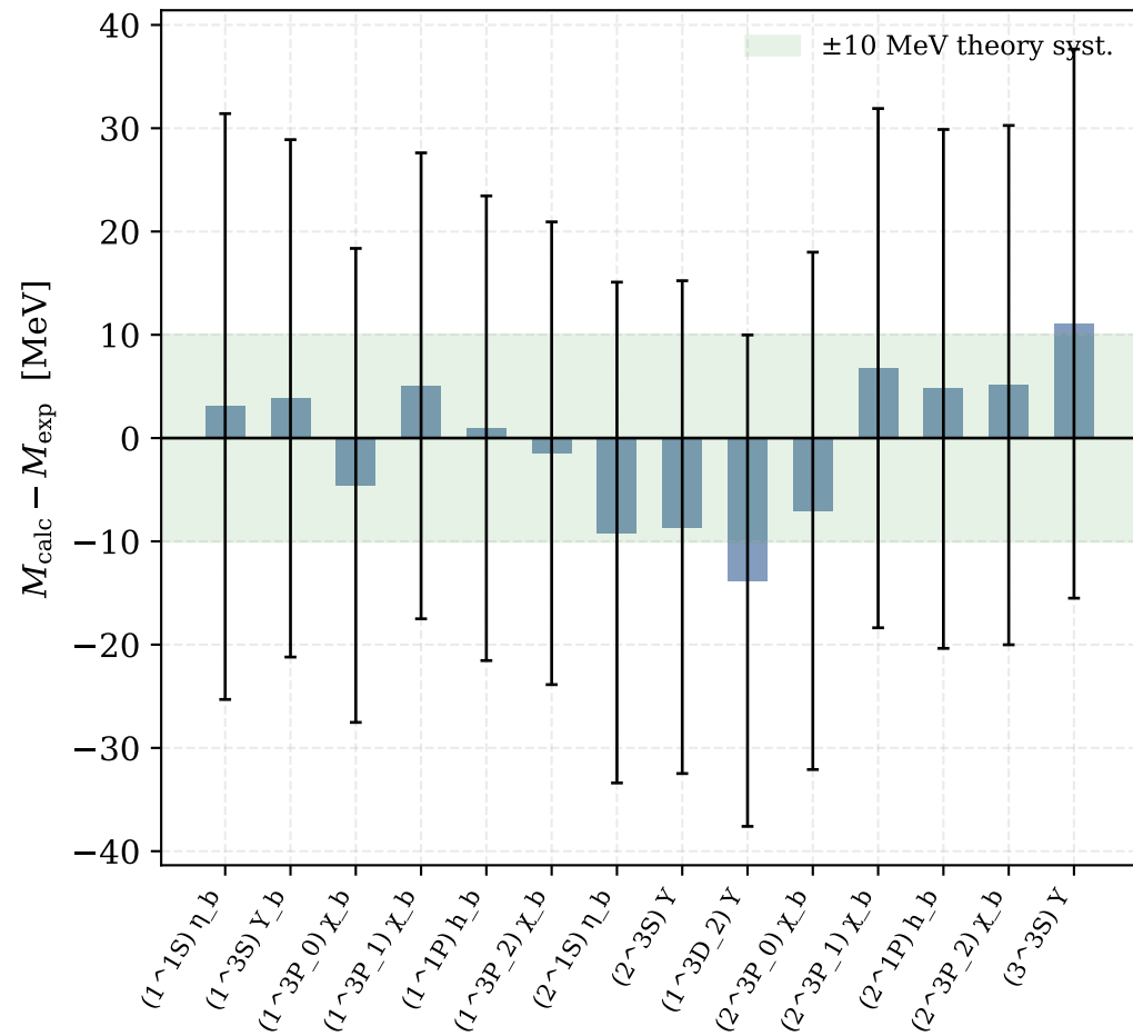
Bottomonium b\bar{b} mass residuals (bars: model uncertainty)
