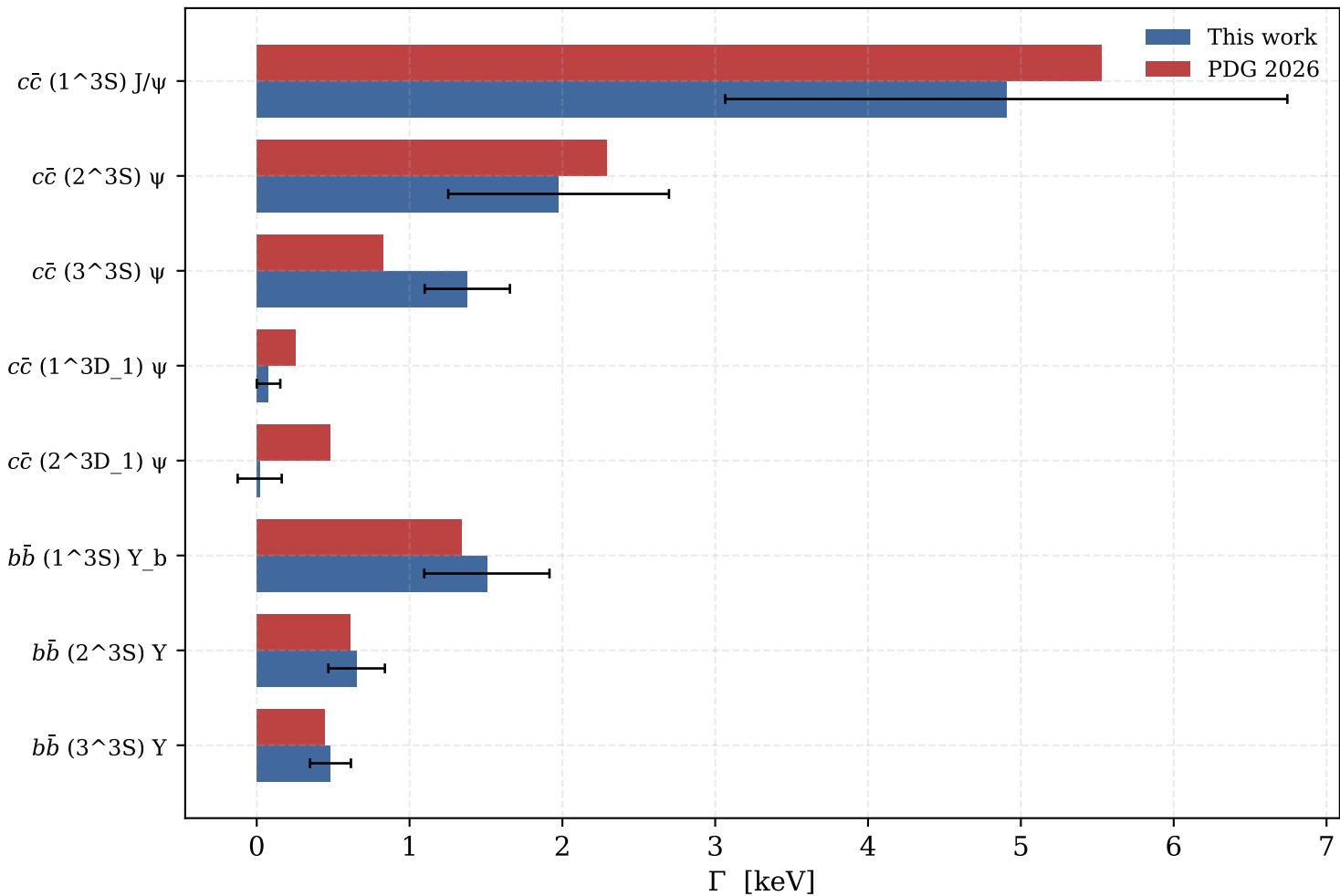
Leptonic V \rightarrow e^+ e^- widths vs. PDG
