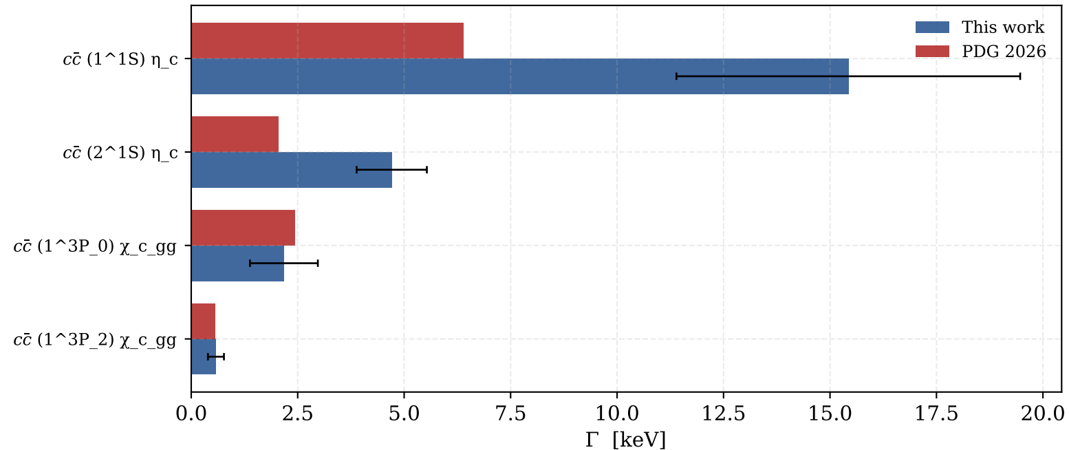
Two-photon P \rightarrow \gamma\gamma widths vs. PDG
