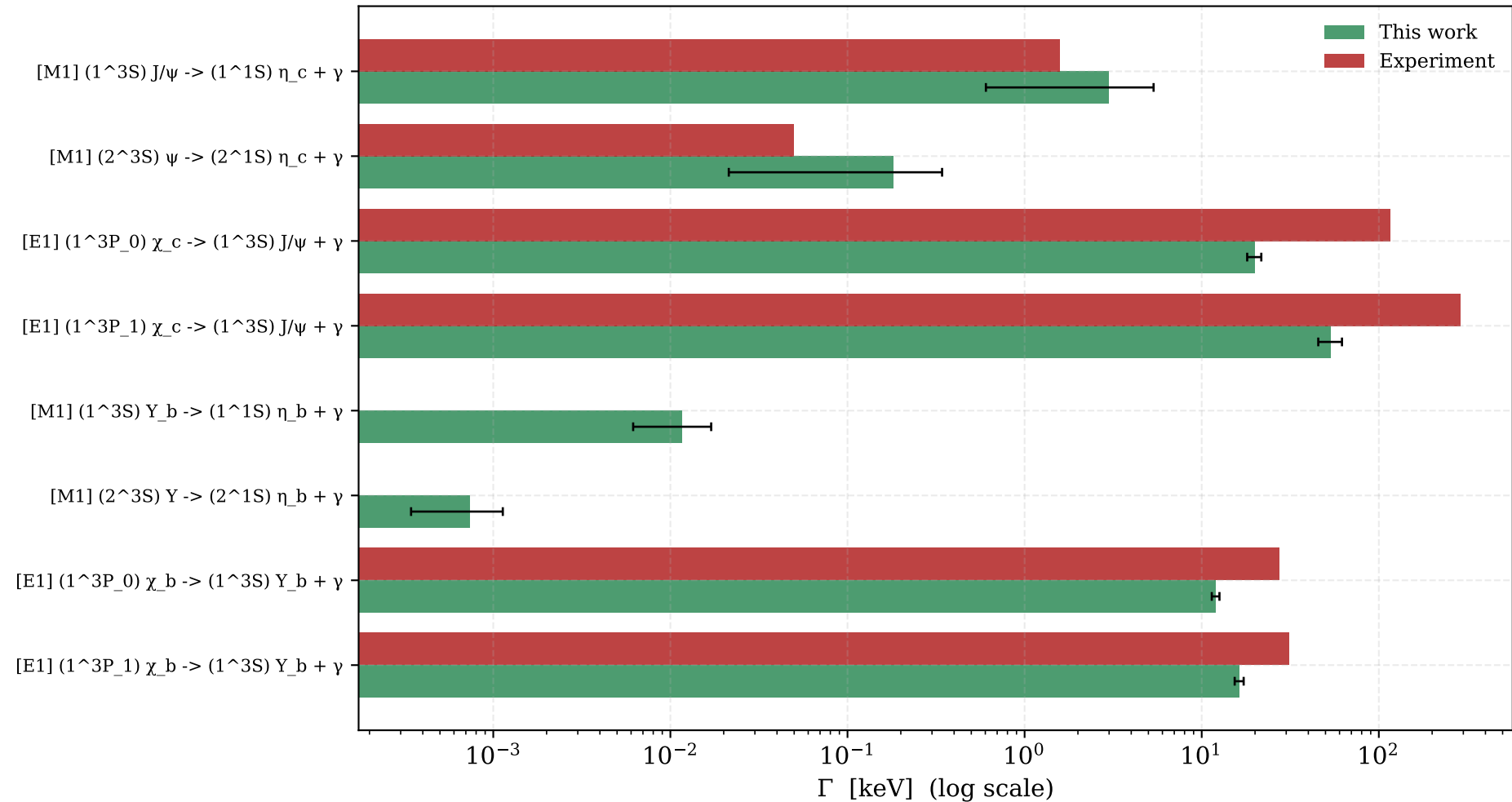
Radiative E1/M1 transition widths vs. experiment
