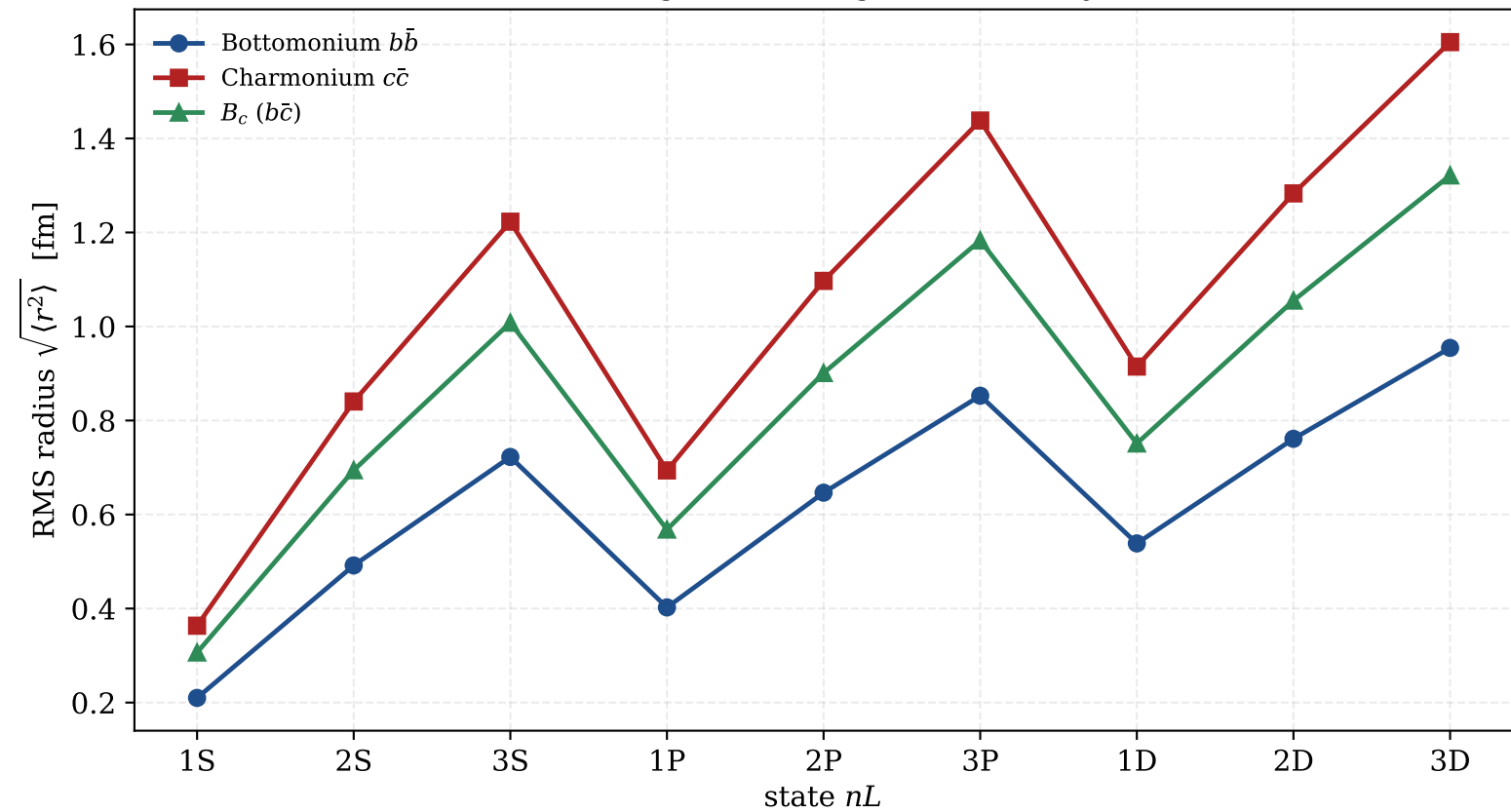
RMS radii: tighter binding for heavier systems
