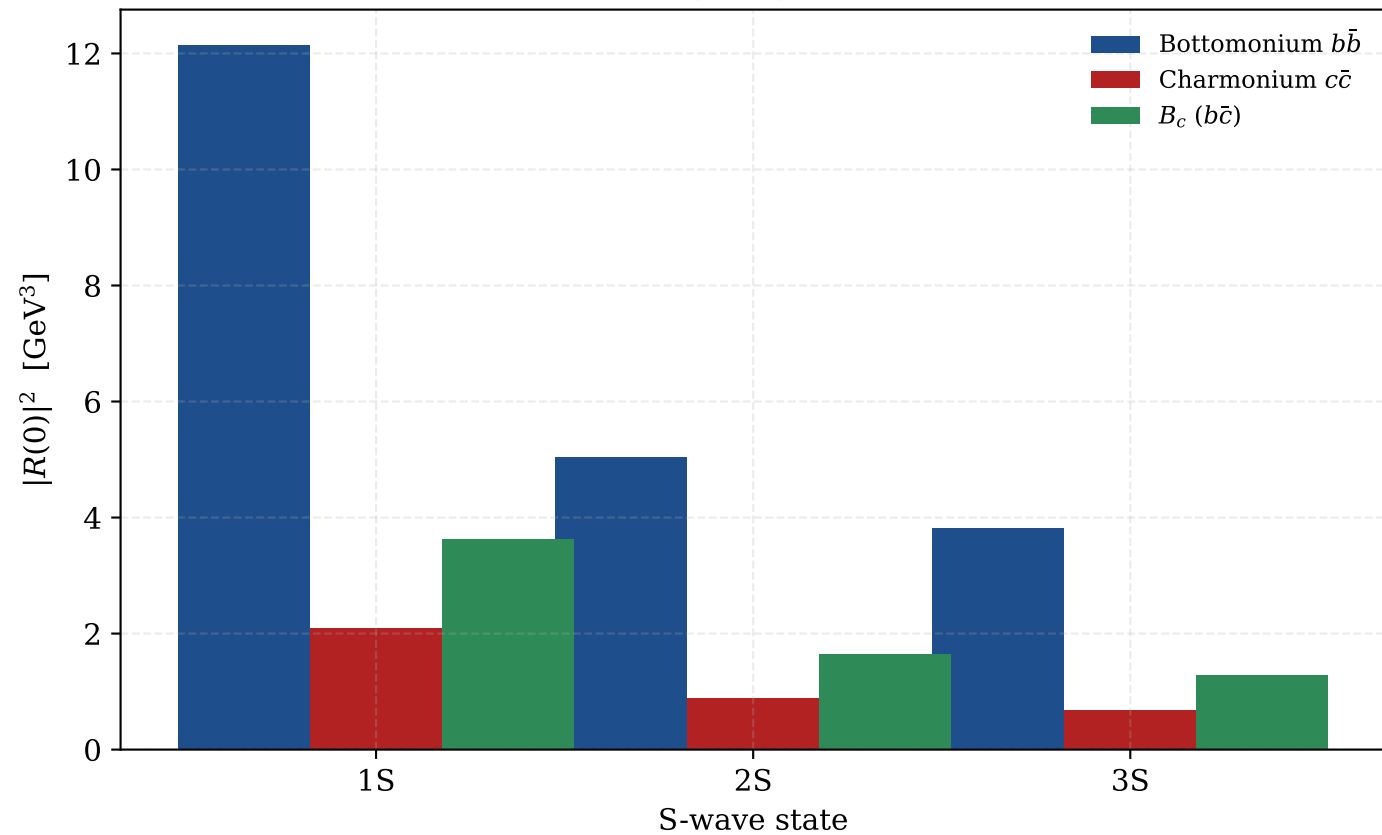
Wavefunction at the origin |R(0)|^2 (drives annihilation widths)
