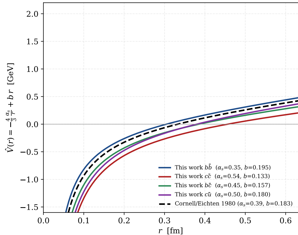
Cornell potential shape vs. the canonical form (unphysical constant offset c removed)
