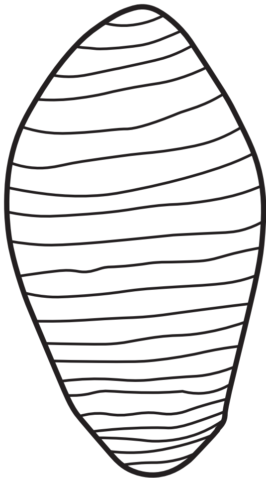
Neanderthal C1
