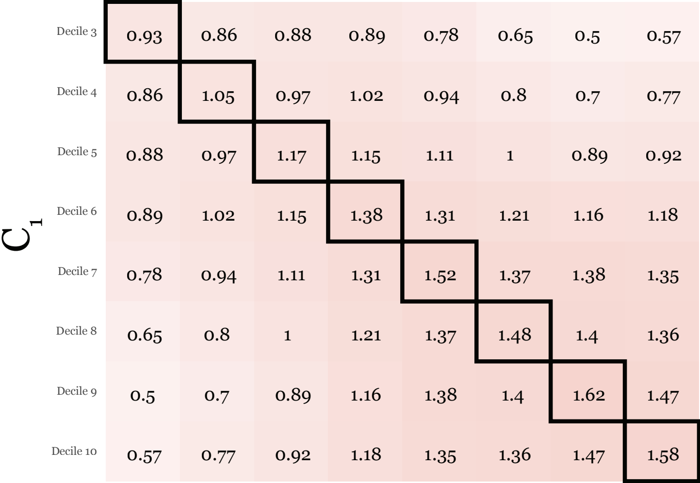
With intraspecific variation
