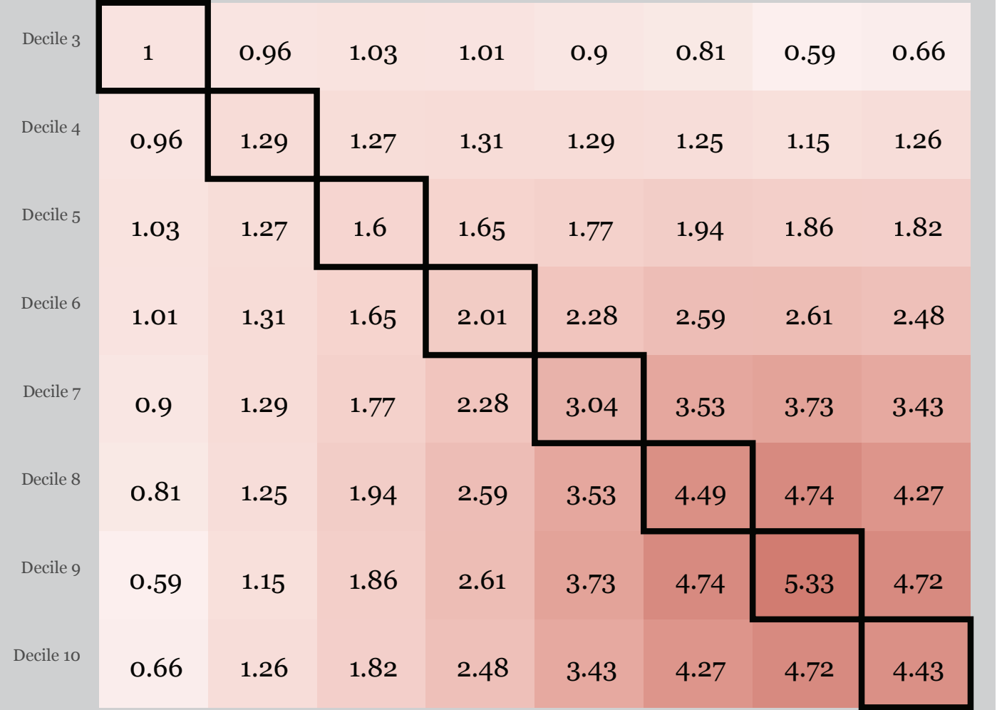
Without intraspecific variation
