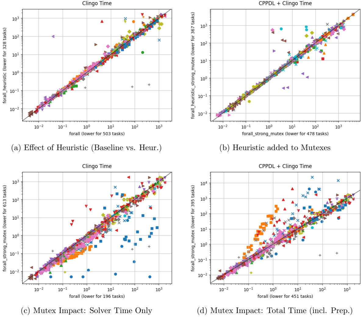
Figure 4.4: Runtime comparison of optimization techniques. Top row: The heuristic shows negligible impact (points on diagonal). Bottom row: Mutexes significantly reduce solver time (c), but preprocessing overhead affects total time on easy instances (d).
