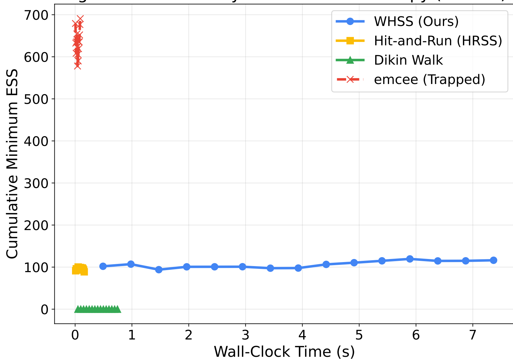
Algorithmic Efficiency in Extreme Anisotropy ( \kappa = 10^4 )
