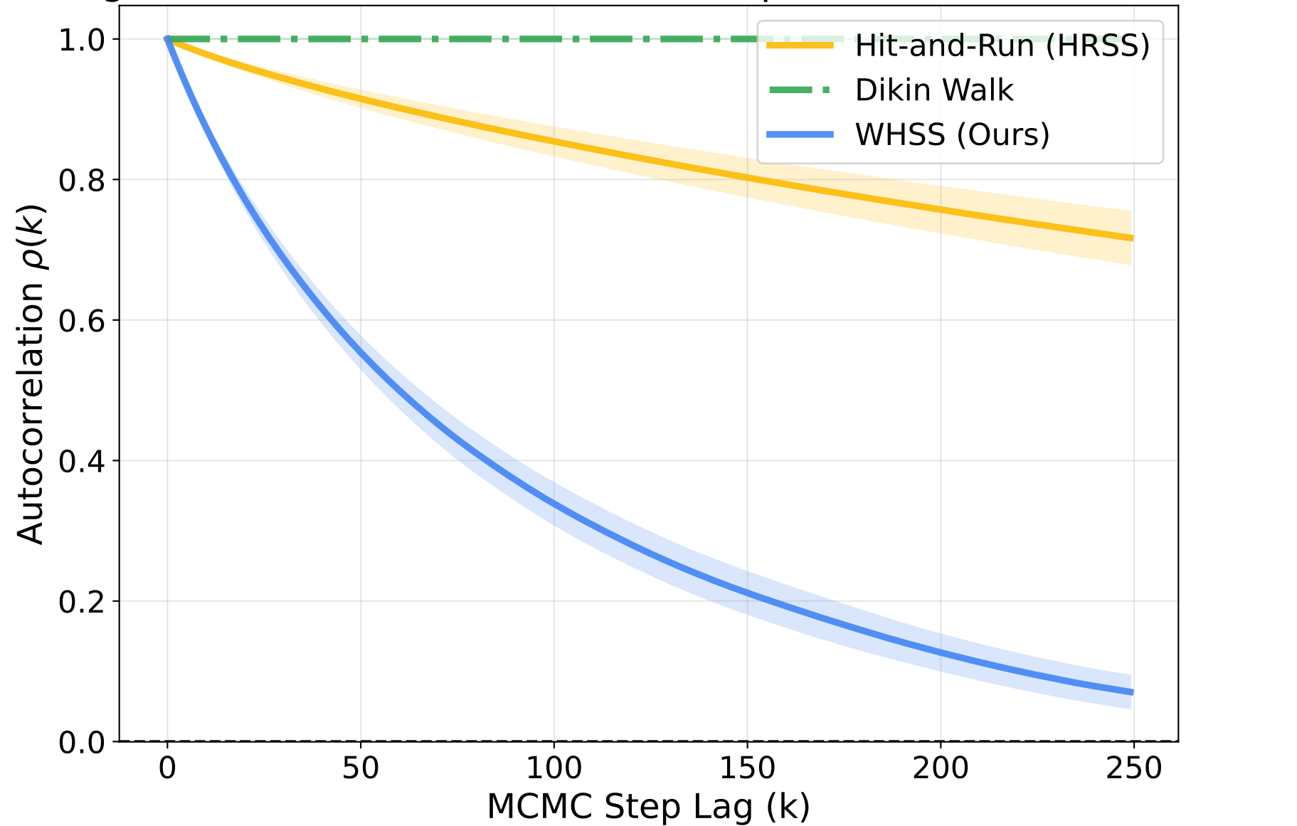
Mixing Autocorrelation in 30D Skewed Space (Cond=1000, 10 Runs)
