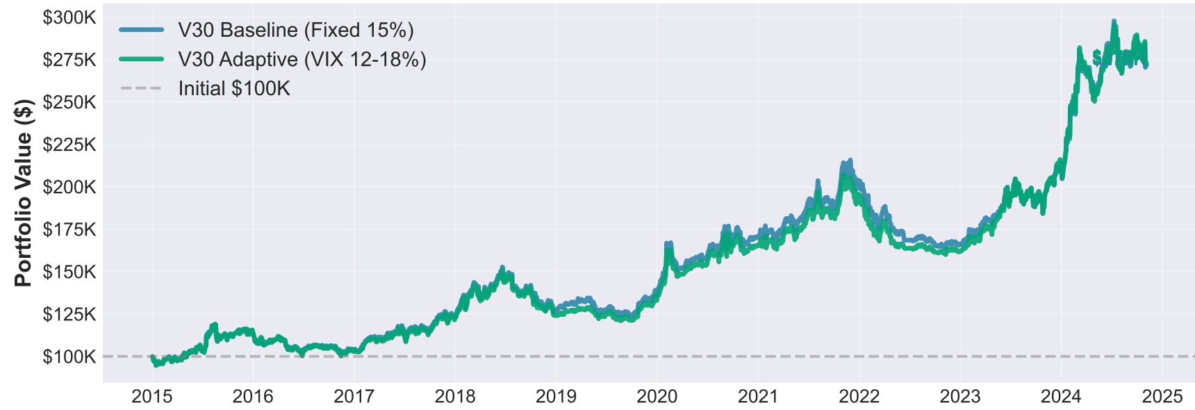
Portfolio Value Over Time (2015-2024)
