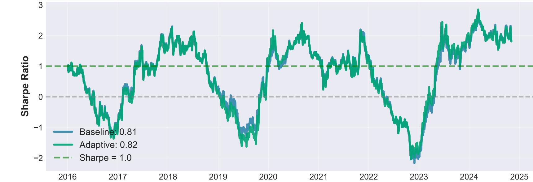
Rolling Sharpe Ratio (252-day)
