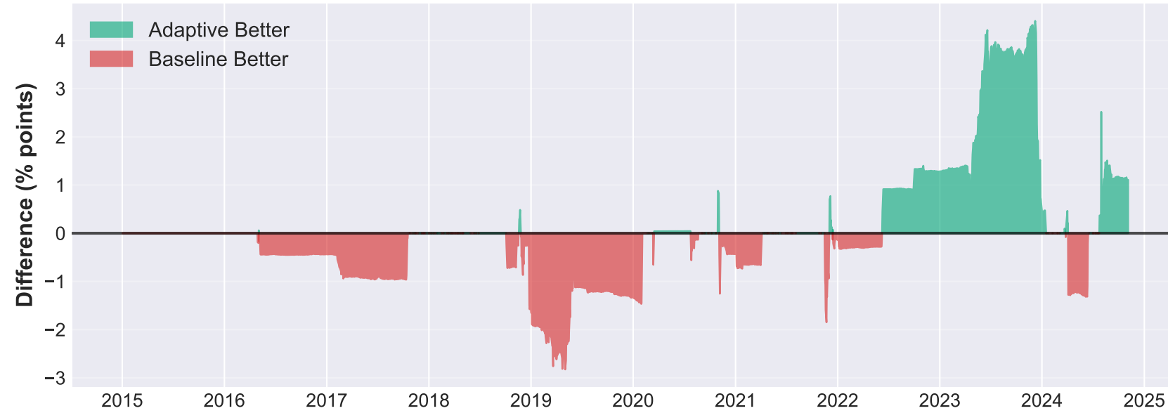
Drawdown Difference (Adaptive - Baseline)
