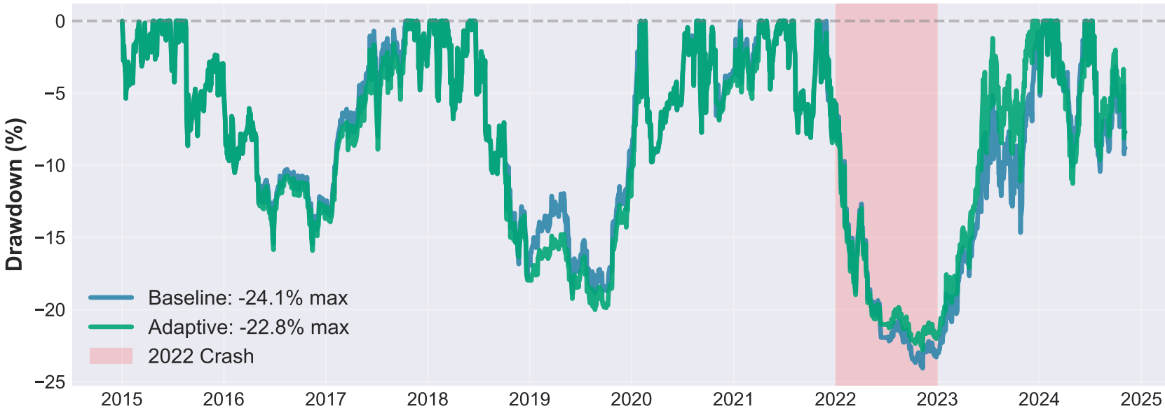
Drawdown Comparison (2022 Highlighted)
