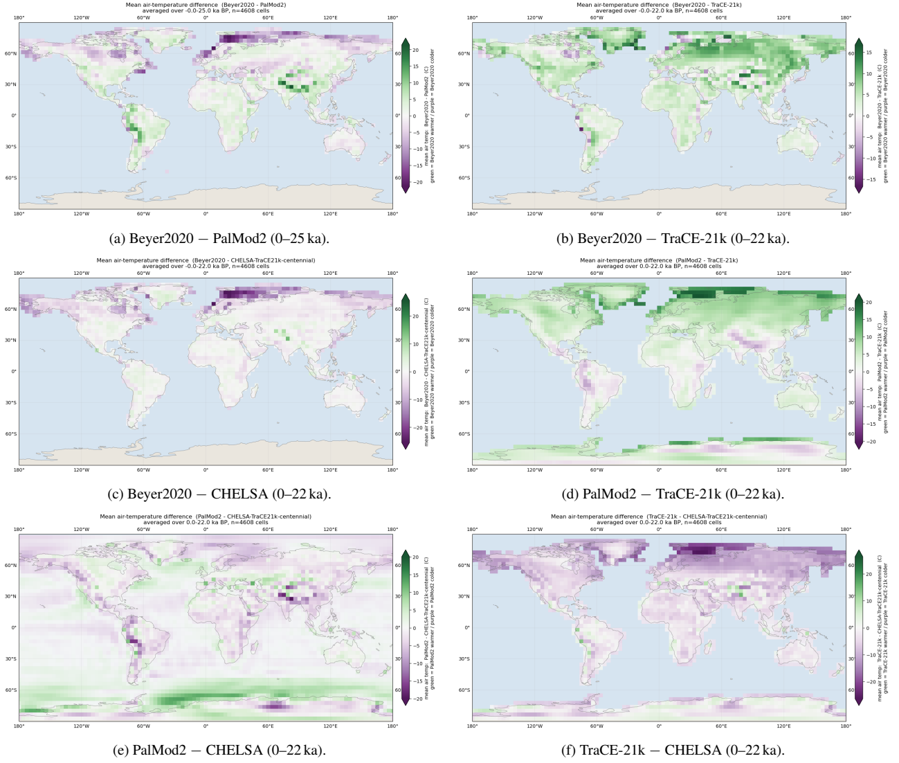
Figure 6. Mean air-temperature differences for all six pairs of the four archives (green = first archive warmer, purple = colder), sampled at the TraCE grid and averaged over each pair’s shared time window.
