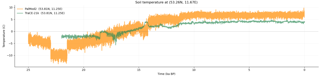
Figure 2. Top-layer soil-temperature time series at the example point for PalMod2 and TraCE-21k (the only two archives with a soil variable).
