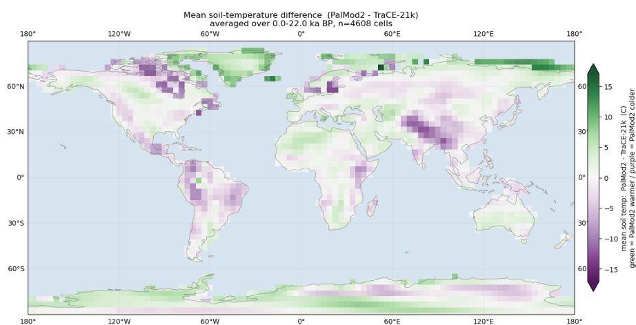
Figure 5. Mean top-layer soil-temperature difference, PalMod2 — TraCE-21k, averaged over the shared 0–22 ka BP window (green = PalMod2 warmer, purple = PalMod2 colder).
