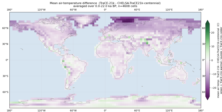
Figure 11. Mean air-temperature difference, TraCE-21k — CHELSA-TraCE21k-centennial (0–22 ka), sampled at the TraCE-21k grid and averaged over the pair’s shared time window (green = first archive warmer, purple = colder).
