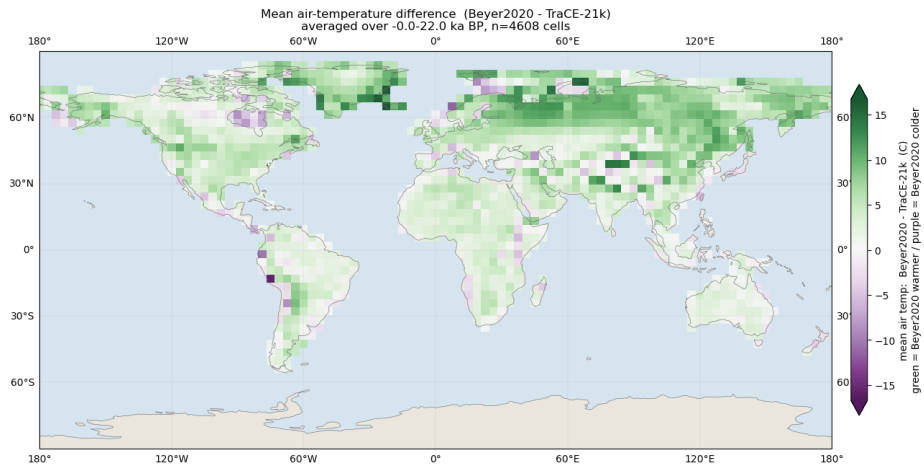
Figure 7. Mean air-temperature difference, Beyer2020 – TraCE-21k (0–22 ka), sampled at the TraCE-21k grid and averaged over the pair's shared time window (green = first archive warmer, purple = colder).
