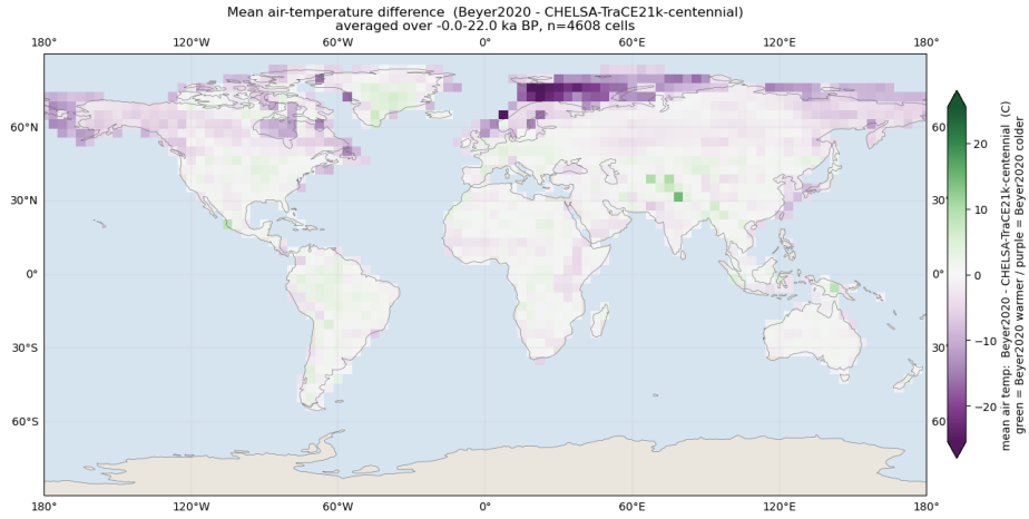
Figure 8. Mean air-temperature difference, Beyer2020 – CHELSA-TraCE21k-centennial (0–22 ka), sampled at the TraCE-21k grid and averaged over the pair’s shared time window (green = first archive warmer, purple = colder).
