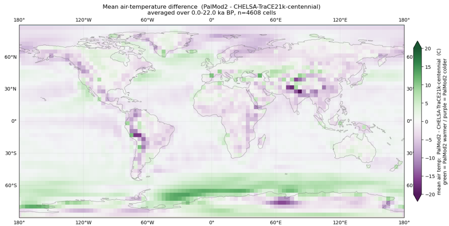
Figure 10. Mean air-temperature difference, PalMod2 – CHELSA-TraCE21k-centennial (0–22 ka), sampled at the TraCE-21k grid and averaged over the pair’s shared time window (green = first archive warmer, purple = colder).
