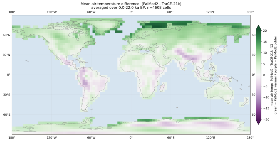
Figure 9. Mean air-temperature difference, PalMod2 – TraCE-21k (0–22 ka), sampled at the TraCE-21k grid and averaged over the pair’s shared time window (green = first archive warmer, purple = colder).
