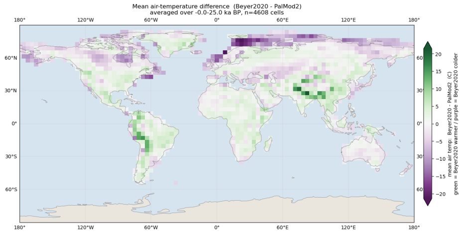
Figure 6. Mean air-temperature difference, Beyer2020 – PalMod2 (0–25 ka), sampled at the TraCE-21k grid and averaged over the pair's shared time window (green = first archive warmer, purple = colder).
